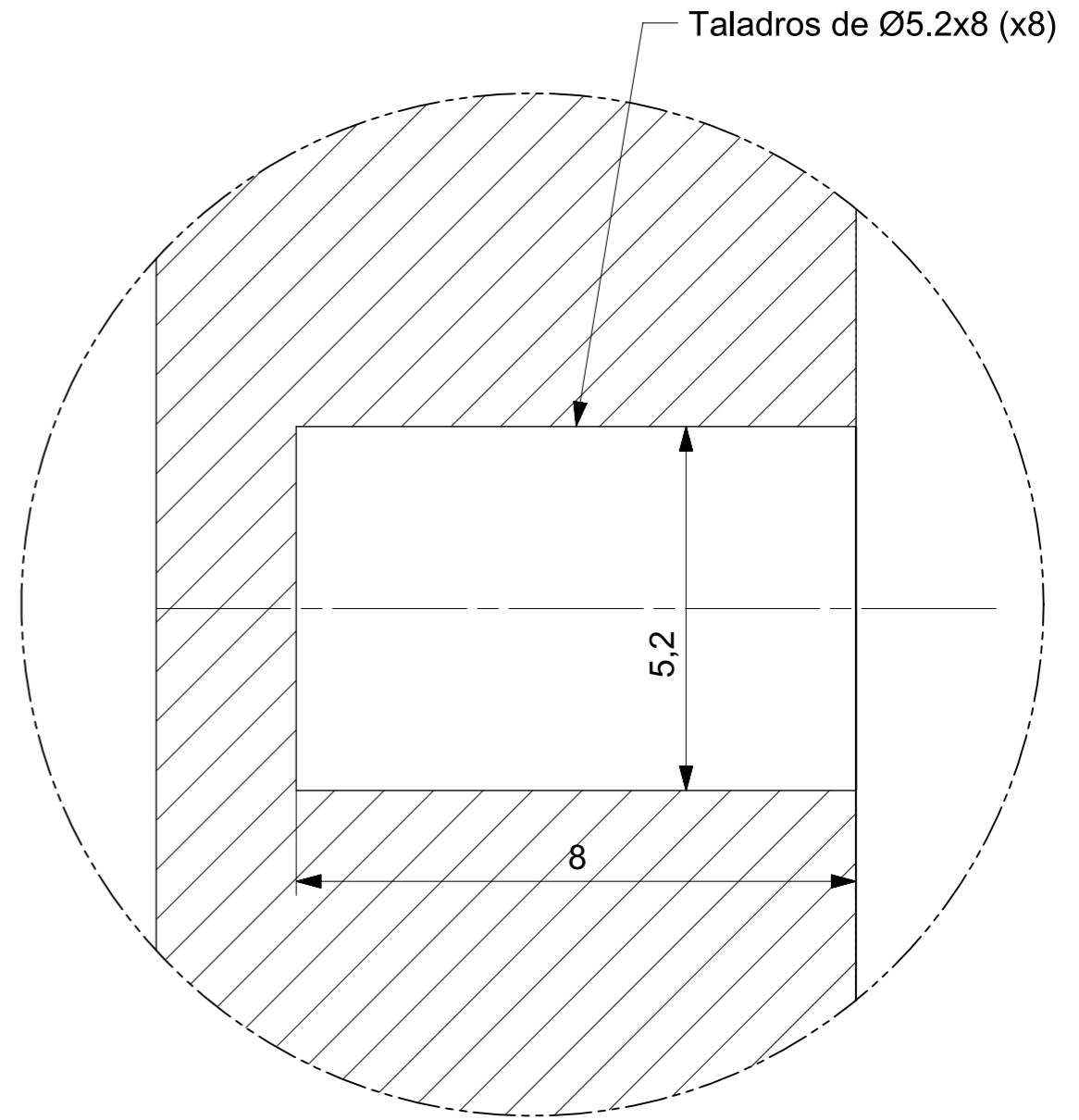
DETAIL C SCALE 10:1
